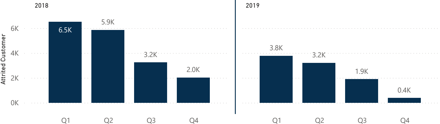
Customer Leave
