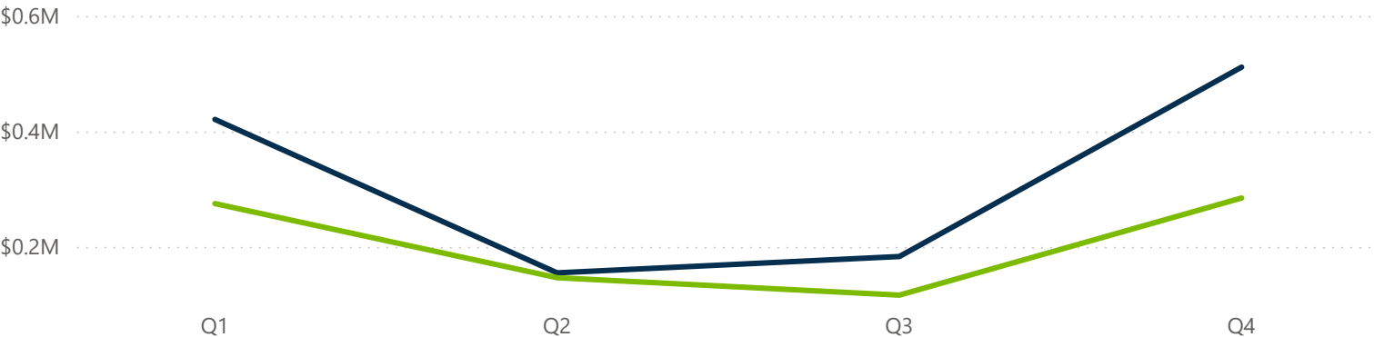
Customer Leave
